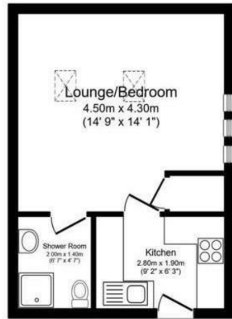
Floor Plan
